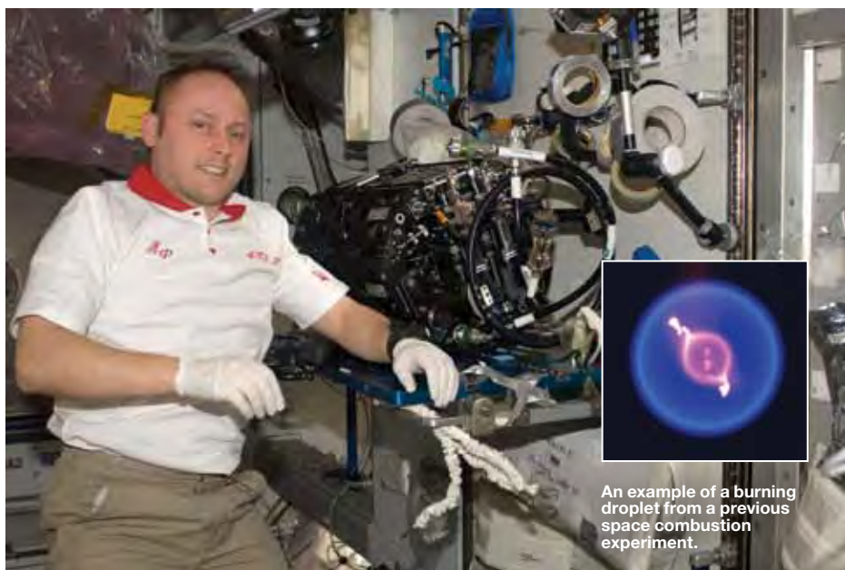
The Multi-User Droplet Combustion Apparatus—Flame Extinguishment Experiment (MDCA-FLEX) [NASA] creates droplets of fuel that ignite while suspended in a containment chamber.
