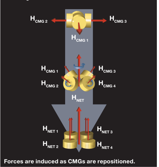
Control Moment Gyroscope gimbals used for orienting the ISS.
