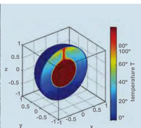
GEOFLOW was the first experiment container processing FSL. The first experiment in the FSL studied a model of liquid core planets.
