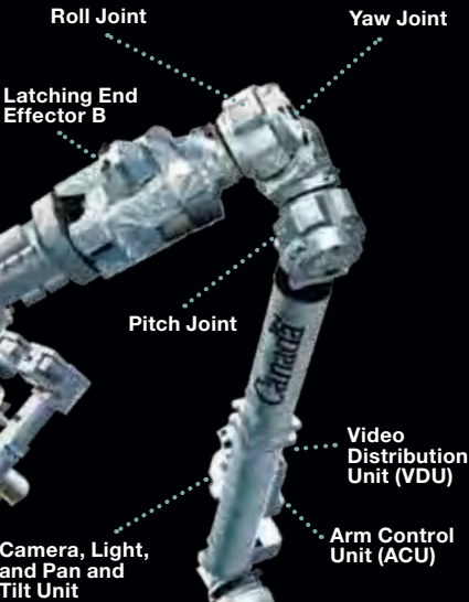
SSRMS during testing.
